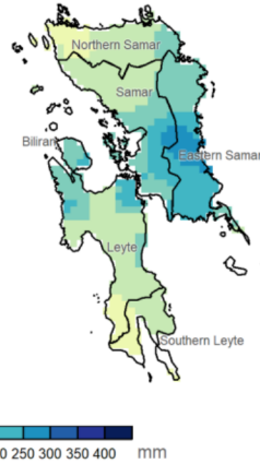
RX5day
